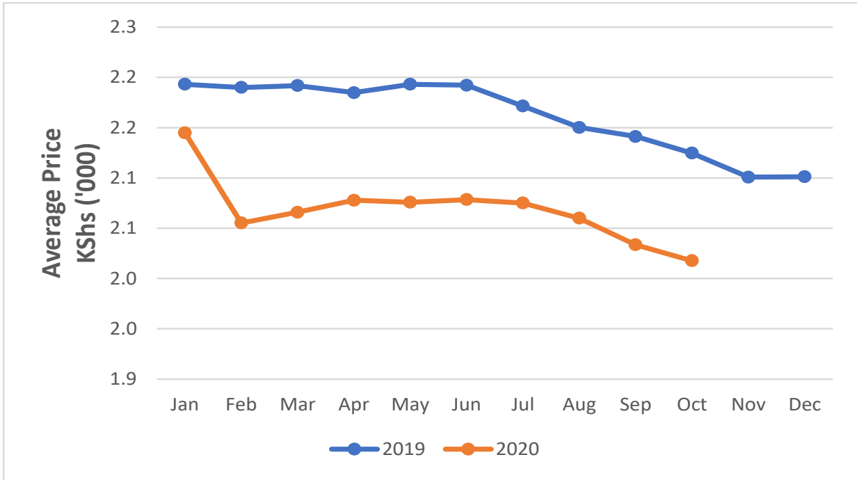
Fig. 8: Average Prices for Liquefied Petroleum Gas in Kenya ('000 KSh per 13 Kg cylinder)
